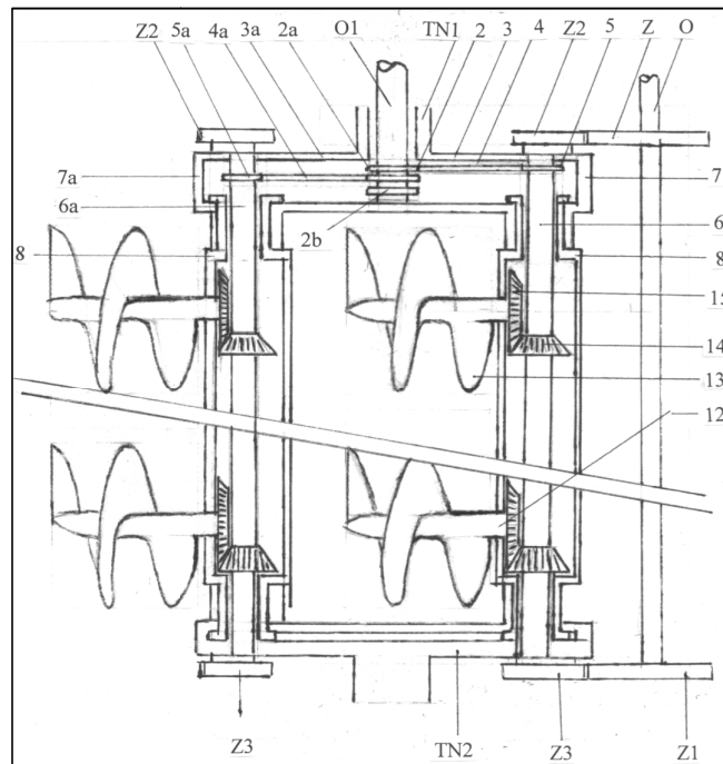
Fig. 2. Accessory machine for monophasic complex agrotechnology Horizontal cross-section through three-beamed bear TN1 and TN2, and bore bearers 8,8a and 8b, and bores 13, with chain transmission 10 (variance 1)
