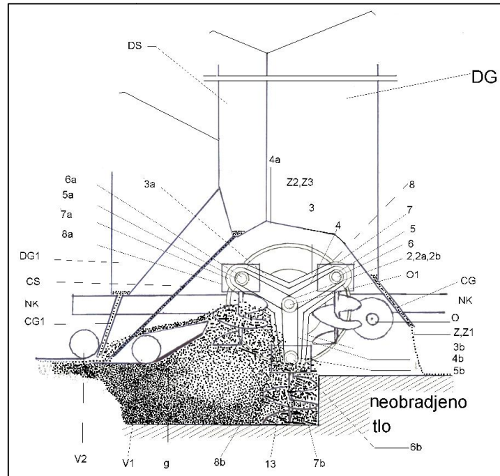
Fig. 1. Accessory machine for single-phase complex agro-technology - vertical cross-section through the triple carrier TN1 - horizontal cross-section through the triple carrier TN1 and TN2, and supports drill bits: 8,8a, 8b and drill bits 13 (variant I, chain link 10)
