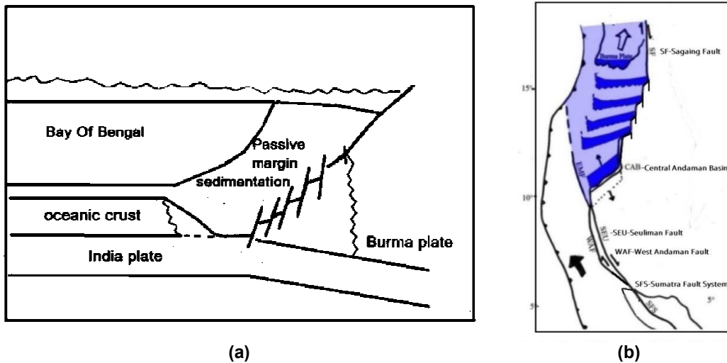
Fig.2.(a).A cross-section showing a passive margin of the western side of the Burma plate.(b) A map showing dispersion model of the Burma plate from the Central Andaman Basin to the north
