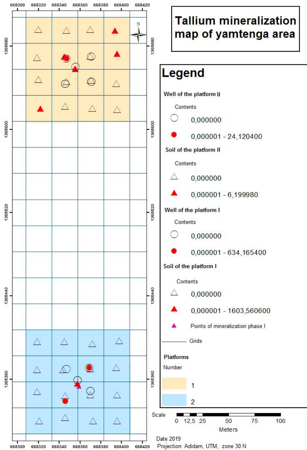
Fig. 9. Spatial distribution of thallium in the soil
