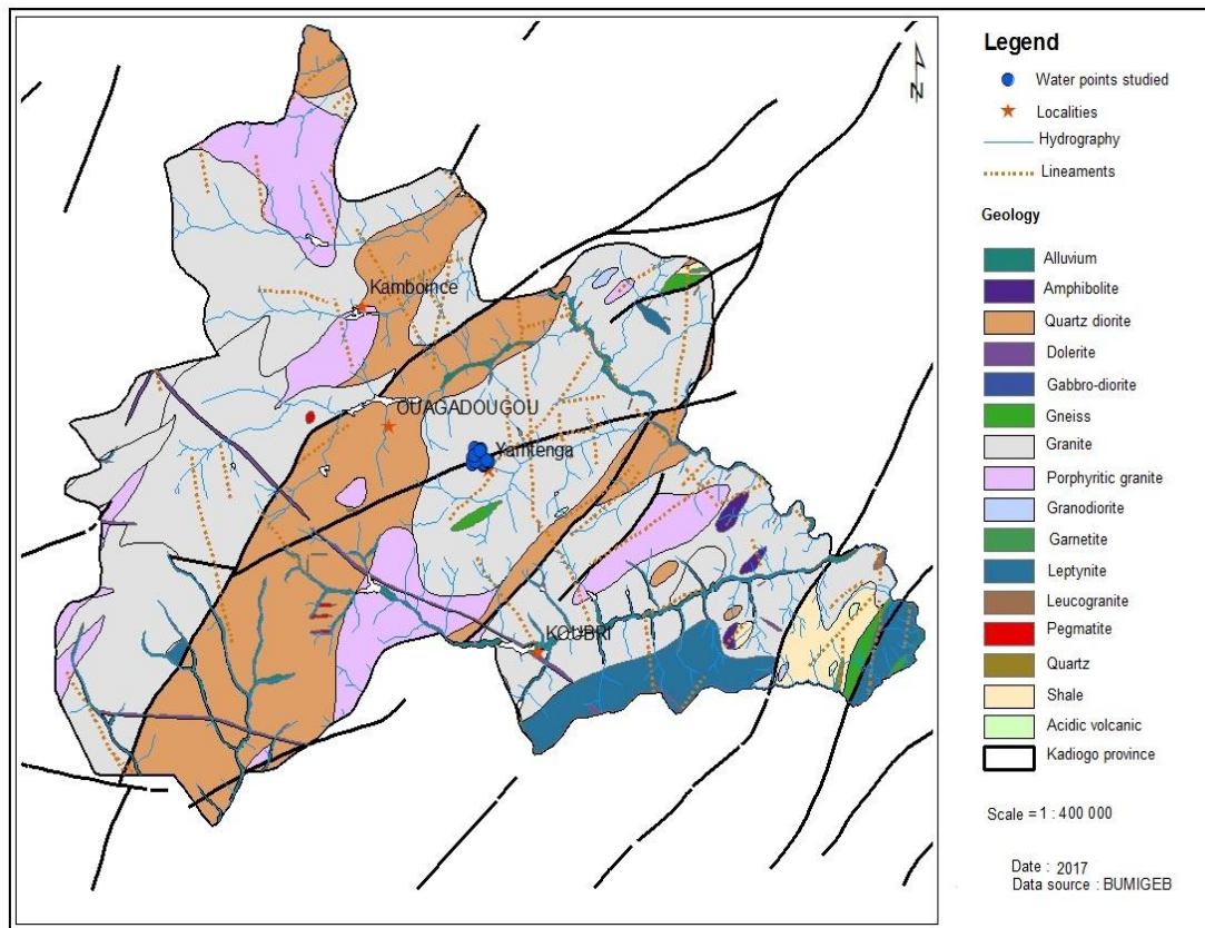
Fig. 1. Geological map of the central region (including the studied area)
