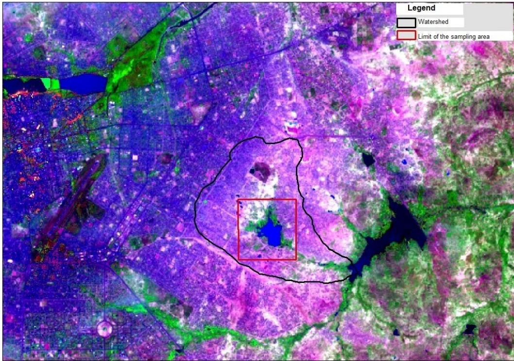
Fig. 5. Landsat image in 2015
