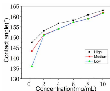
Fig. 7. The influence of concentration on wettability
