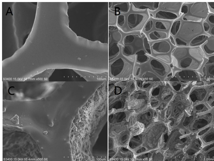
Fig. 9. SEM analysis of sponge surface (A and B are SEM images of the pristine sponge; C and D are SEM images of superhydrophobic sponge)
