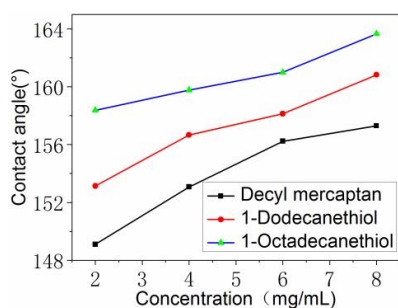
Fig. 8. The effect of the type of mercaptan on the wettability of materials
