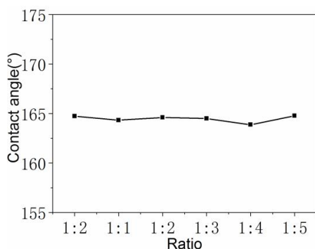
Fig. 2. The influence of the ratio on water contact angle
