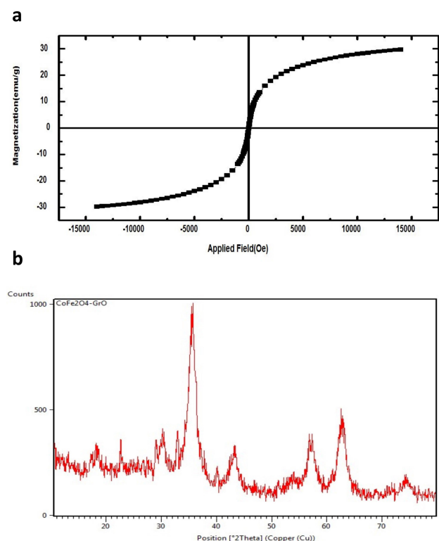
Figure 2. VSM diagram a) and XRD pattern b) of \text{CoFe}_2\text{O}_4 -GO nanocomposite.
