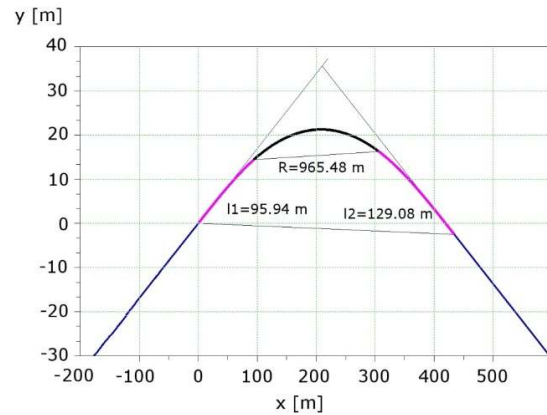
Fig. 2. Variant of the route in horizontal arc of radius R = 965.48 m together with two transition curves of length l_1 = 95.94 m and l_2 = 129.08 m (non-isometric scale)
