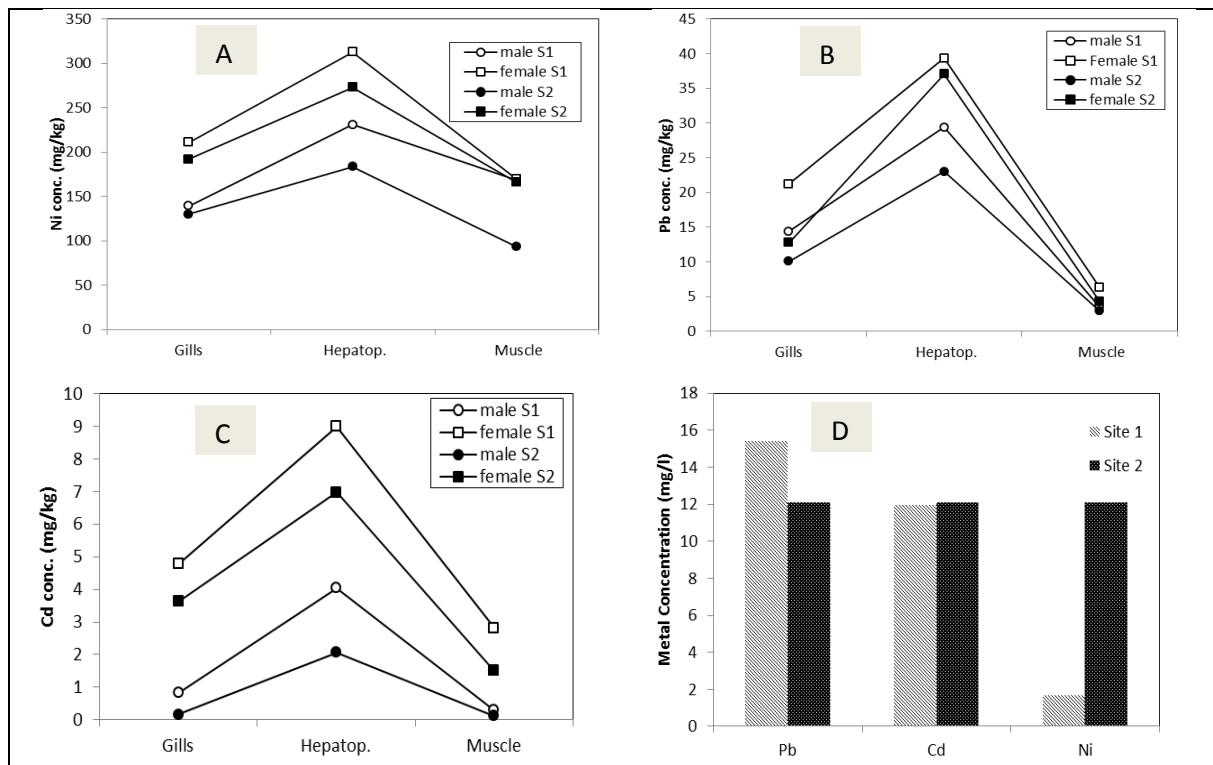
Fig. 3. Metals in tissue of Callinectes sapidus and water obtained from Iko River (A) Ni in C. sapidus (B) Pb in C. sapidus (C) Cd in C. sapidus (D) Metals in water of Iko river
