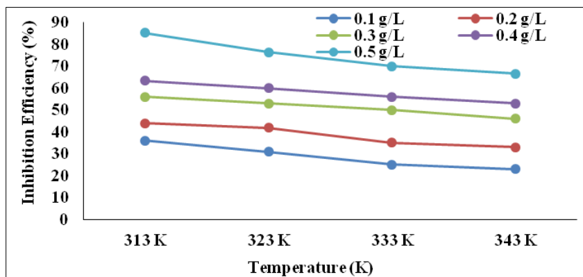
Fig. 5. Variation of inhibition efficiency of AHL inhibitor with temperature at various concentrations
