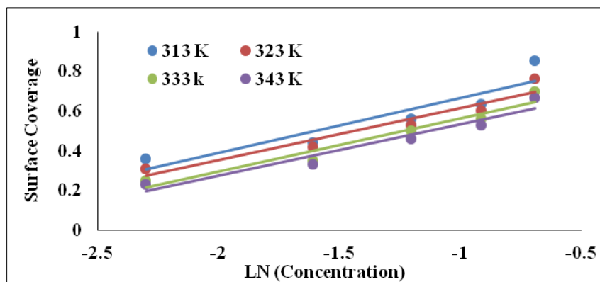
Fig. 8. Temkin Adsorption Isotherm for Mild Steel in 1.0 M HCl Solution in the Presence of AHL Extract
