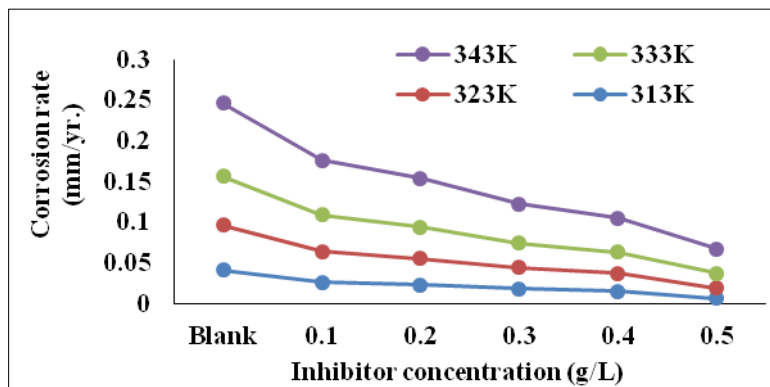
Fig. 3. Variation of corrosion rate with AHL concentration at elevated temperatures
