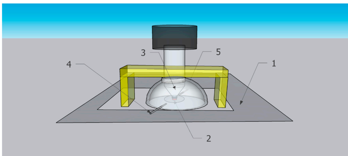
Figure 3. Scheme of spectroscopic mini-chamber installed on baseplate of the FTIR spectrometer with existing ATR assembly.
