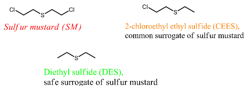
Figure 1. Sulfur mustard and its surrogates with similar structure and properties.
