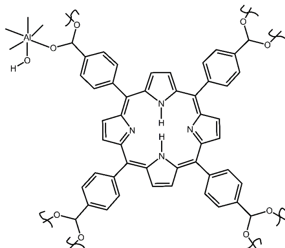
Figure 2. The simplified structural unit of starting compound 2 porphyrin aluminum MOF (Al-MOF-TCPPH 2 ).
