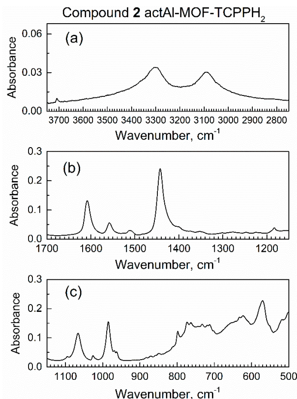
Figure 4. Major ranges of the in situ ATR-FTIR spectrum of compound 2 actAl-MOF-TCPPH 2 in spectroscopic mini-chamber in flow of dried air: (a) high wavenumbers, (b) the mid-IR range, (c) low wavenumbers range.
