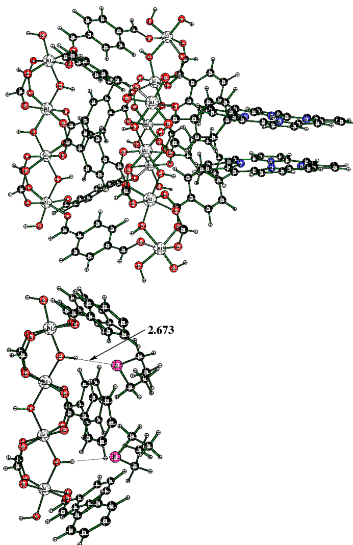
Figure 12. (Top) The full cluster Al-TCPPH 2 without DES molecules. (Bottom) The cutout of cluster “2DES@Al-TCPPH 2 ” with S---HOAl binding motif, where two DES molecules interact with HOAl sites.
