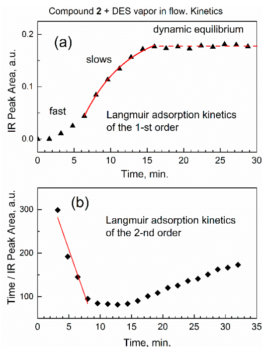
Figure 8. Kinetic analysis of DES sorption based on integrated IR absorbance (peak area) of antisymmetric \text{CH}_2 stretch vibration at 2965\text{ cm}^{-1} . (a) Timescale of the first-order rate law; (b) timescale of the second-order rate law.
