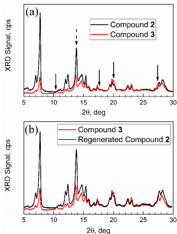
Figure 13. Powder XRD patterns. (a) Compound 2 (sorbent) vs. compound 3 (adsorption complex); (b) compound 3 vs. regenerated compound 2.
