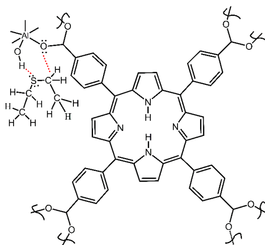
Figure 10. Scheme of bonding of DES molecule to O–H and carboxylate groups in compound 2 .
