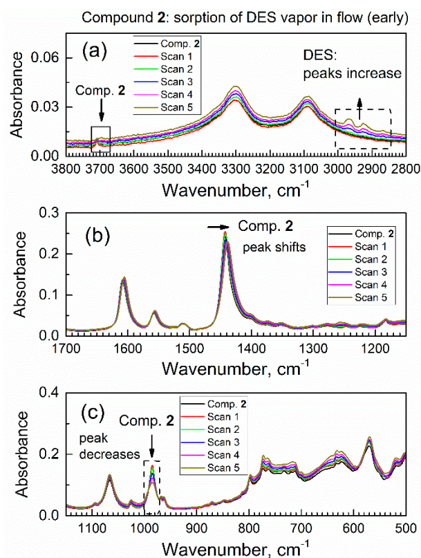
Figure 6. The first set (0–9.6 min) of in situ time-dependent ATR-FTIR spectra of compound 2 in flow of DES vapor in dried air: (a) high wavenumbers range, (b) the mid-IR range, (c) low wavenumbers range.
