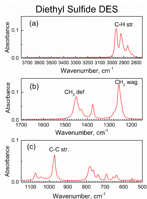
Figure 5. Major ranges of the ATR-FTIR spectrum of liquid DES: (a) high wavenumbers range, (b) the mid-IR range, (c) low wavenumbers range.
