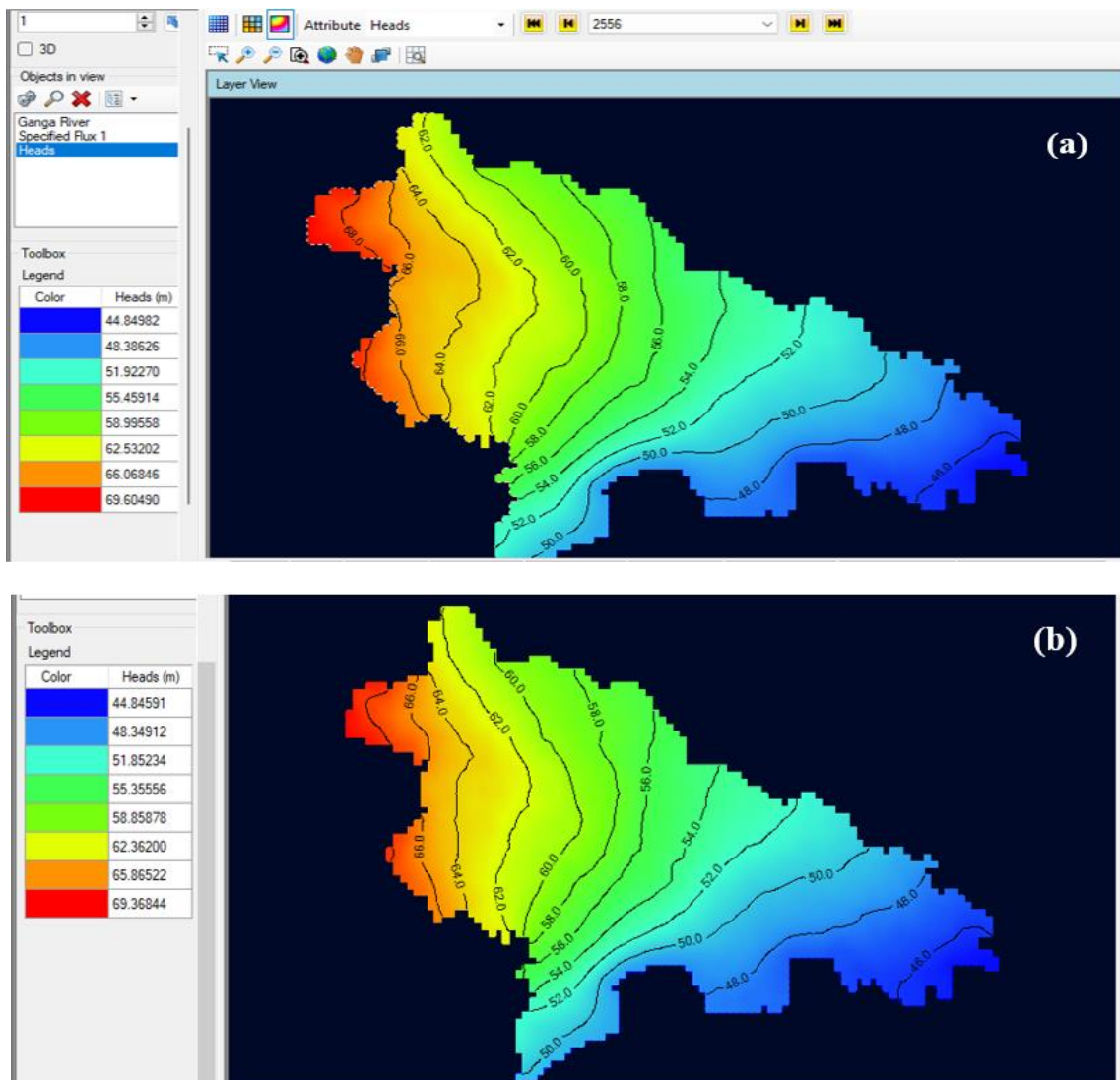
Fig. 5. Predicted Groundwater Level heads (a) at 0 th day of prediction and (b) after 5 years (4748 days)
