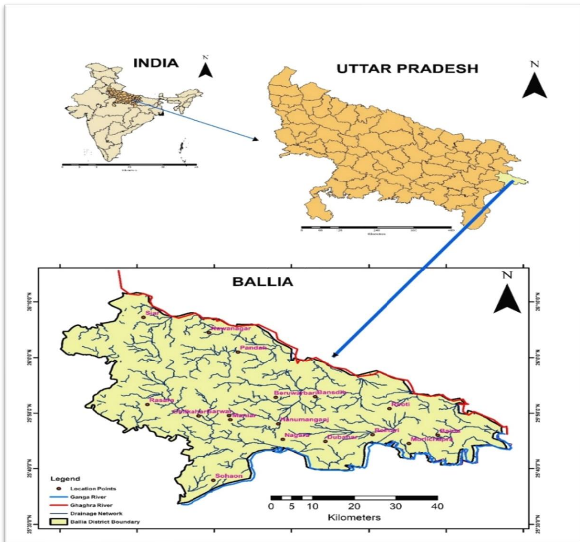
Fig. 1. Location map of the study area (Ballia District, Uttar Pradesh)
