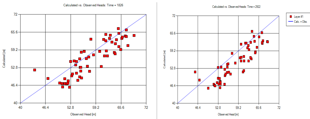
Fig. 4. Scatter-Plot between observed and calculated heads for unconfined aquifer during (A) Calibration; (B)Validation
