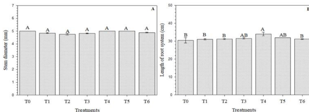
Fig. 6. Length of the root system ( E. contortisiliquum ) at 105 days of age, in different methods of overcoming dormancy. T0: Control; T1: Mechanical scarification with a rasp; T2: Mechanical scarification with electric welding apparatus, T3: Mechanical scarification with cutting pliers; T4: Chemical scarification with sodium hydroxide 30% for 25 minutes; T5: Chemical scarification with sodium hydroxide 30% for 30 minutes; T6: Immersion in water 100°C for 7 minutes
