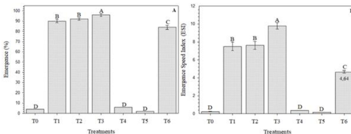
Fig. 5. Emergence percentage (A) and Emergence Speed Index (B) (24 days after sowing) of Earpod tree seeds ( E. contortisiliquum ) with different dormancy overcoming methods. T0: Control; T1: Mechanical scarification with a rasp; T2: Mechanical scarification with electric welding apparatus; T3: Mechanical scarification with cutting pliers; T4: Chemical scarification with sodium hydroxide 30% for 25 minutes; T5: Chemical scarification with sodium hydroxide 30% for 30 minutes; T6: Immersion in water 100 °C for 7 minutes
