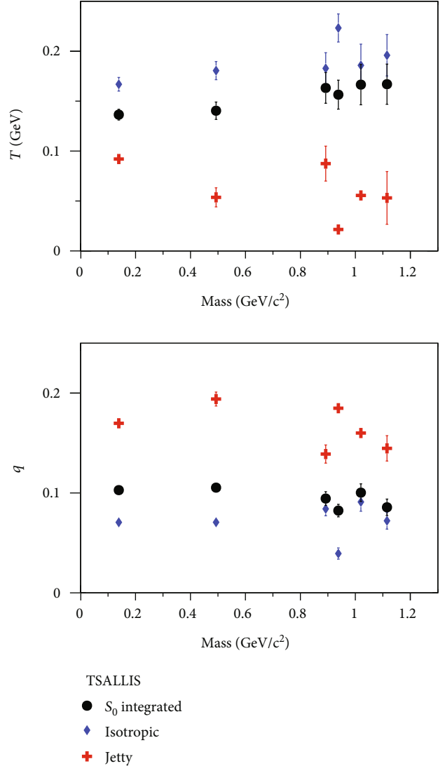
FIGURE 10: (Color online) Mass dependence of T and q in different sphericity classes for the highest multiplicity class.
