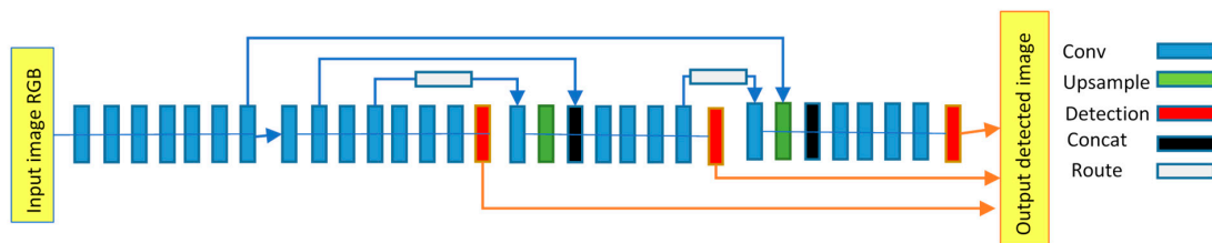
Figure 2. Block diagram of MangoYOLO model.
