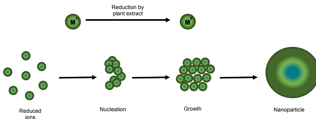
Fig. 4. Steps of formation of metallic nanoparticles [104]
