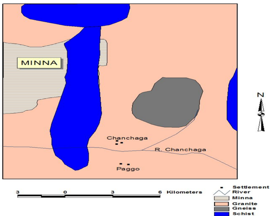
Figure 2. Geological map of parts of Minna (Source: NGSA, 200)
