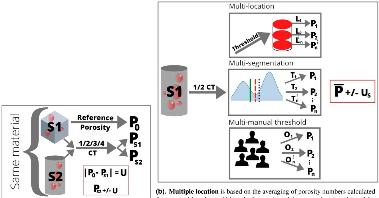
(a). Single scan of two samples based on the comparison of the reference sample with known porosity with an already acknowledged previous porosity measure for uncertainty estimation. (b). Multiple location is based on the averaging of porosity numbers calculated from several locations within a single sample and the uncertainty is estimated from the standard deviation between them. Multi-segmentation is based on the same calculation with different multiple segmentation from the whole sample calculated by an algorithm and averaged. Multiple manual threshold is based on several operators visual choice from one specific slice.
