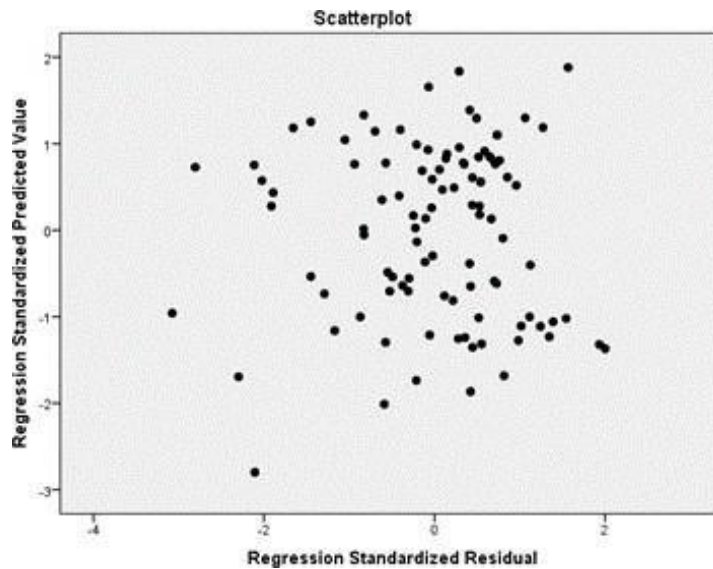
Fig. 2. Homoscedasticity test
