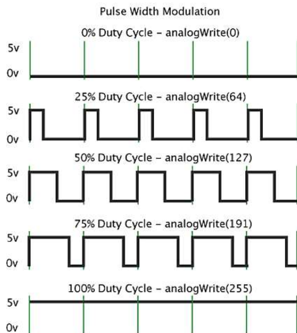
Fig. 5. PWM examples in Arduino [Error! Bookmark not defined.]
