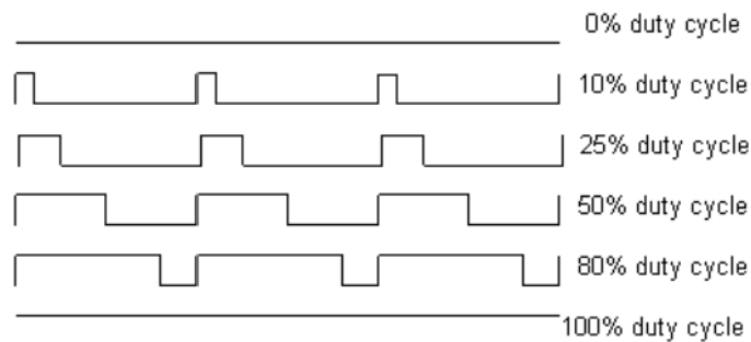
Fig. 4. PWM duty cycles [24]
