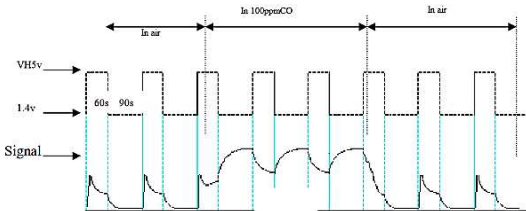
Fig. 6. Heating cycle requirement for MQ sensors [21]
