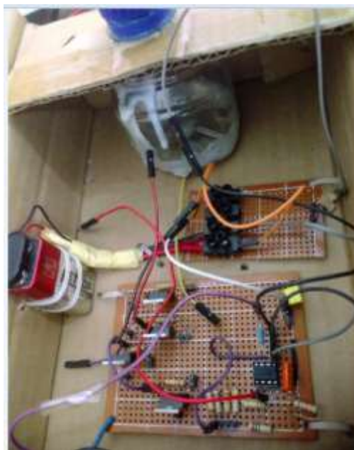
Fig. 9. Prototype with 4 FET for PWM
