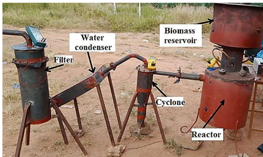
Fig. 1. Picture of the gasifier
