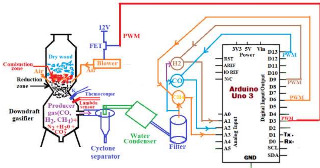
Fig. 7. MQ gas sensors PWM drivers overview
