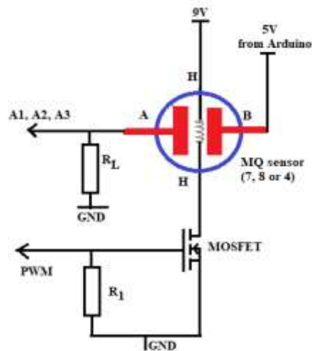
Fig. 3. PWM heating circuit for a MQ sensor
