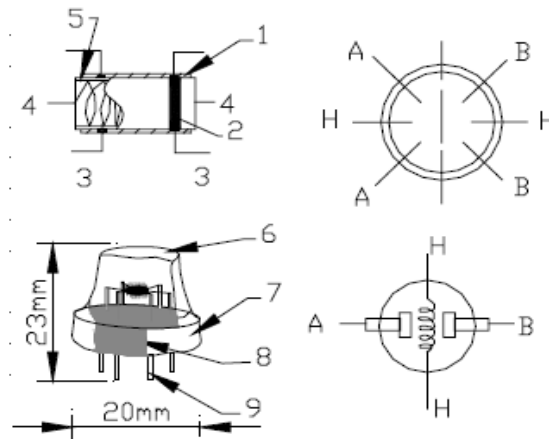
Fig. 2. MQ gas sensors structure [21]
