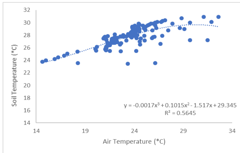
Fig. 6. Correlation between air and surface temperature for inactive solar period
