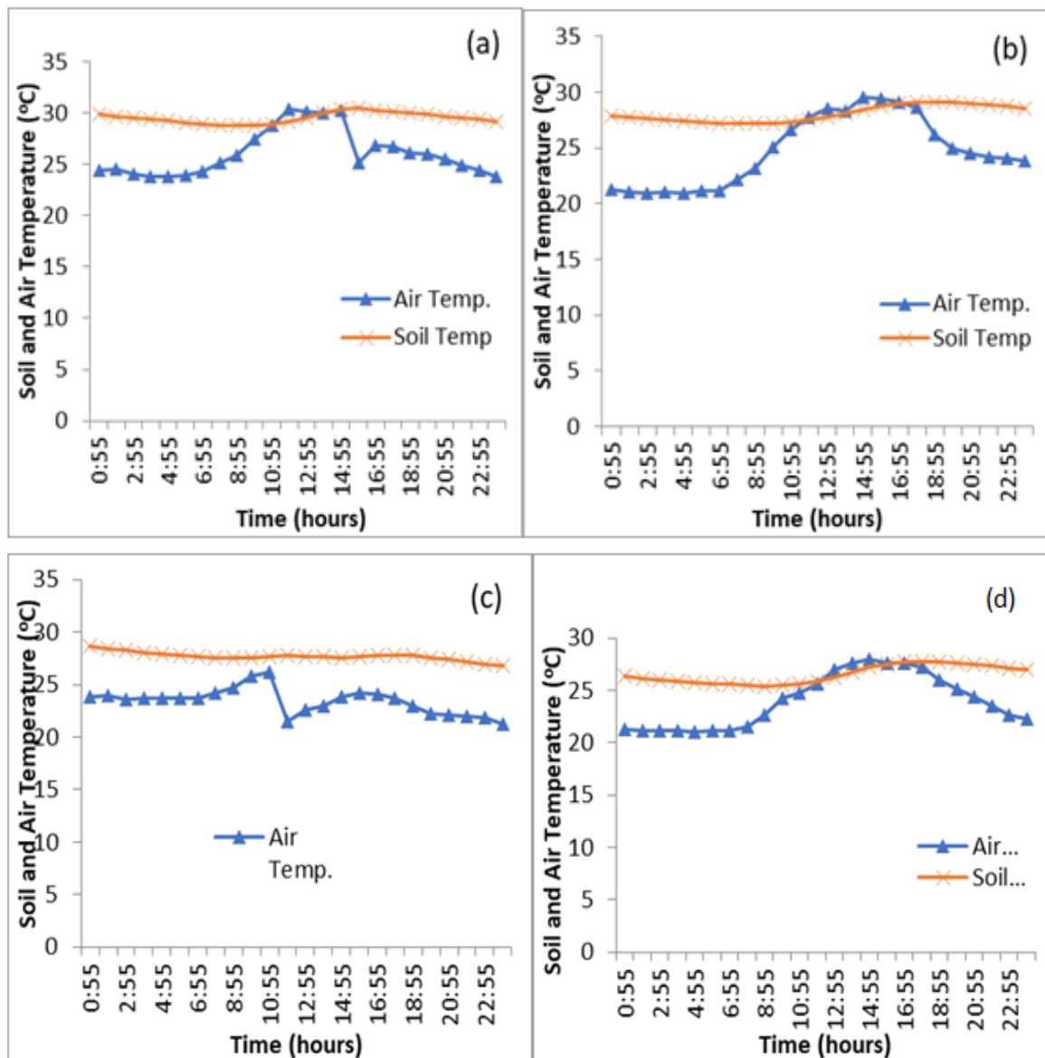
Figs. 3(a-d). Diurnal variation of soil and air temperature during the wet months; (a) May, (b) June, (c) July, (d) August
