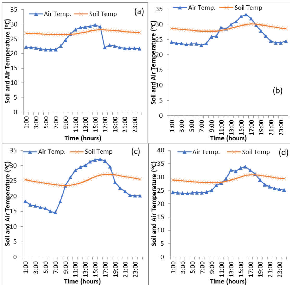
Figs. 4(a-d). Diurnal variation of soil and air temperature during the dry months; (a) November, (b) December, (c) January, (d) February
