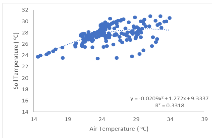
Fig. 5. Correlation between air and surface temperature for inactive and active solar periods
