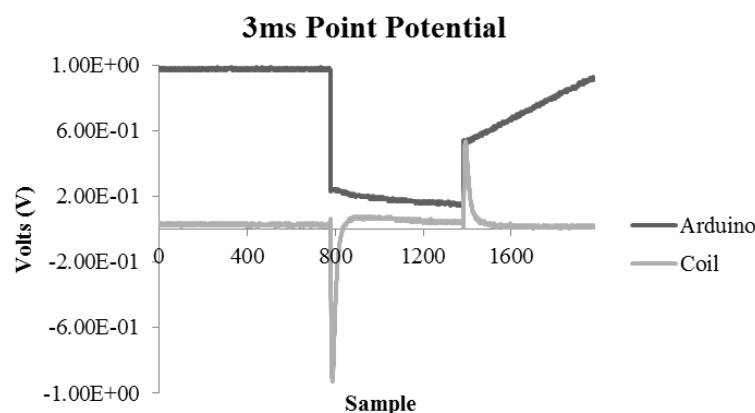
Figure 2. The 2D representation of the 3 ms point durations measured at the level of the Arduino (dark line) and coil (light line) that composed the shape of the field generated within the toroids. The other point durations were similar in shape but were presented for either 1 ms or 2 ms. Here, the x-axis represents samples recorded by an Agilent Technologies MSOX3012A oscilloscope where the time equivalent between peaks is equal to 3 ms.
