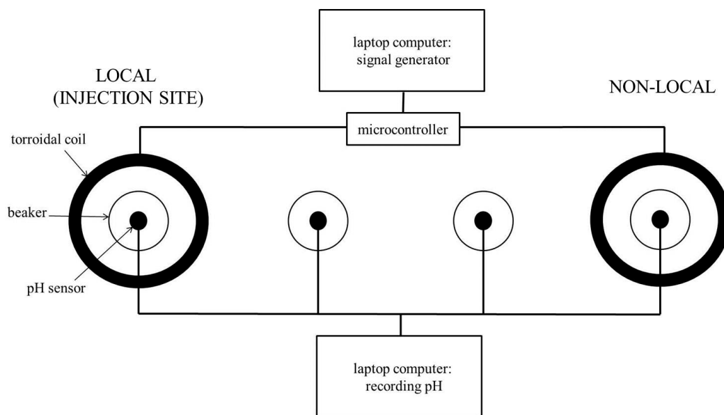
Figure 1. Schematic of the apparatus employed to produce “entanglement” or “excess correlation” in pH shifts within two separate containers of water. The dark circles refer to the toroids that generate the shared fields with changing angular velocities. The two circles representing beakers in the center were “controls” to ensure there were no indirect field effects upon pH shifts.
